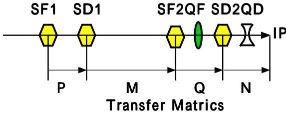
Figure 3: New Final Focus Optics
