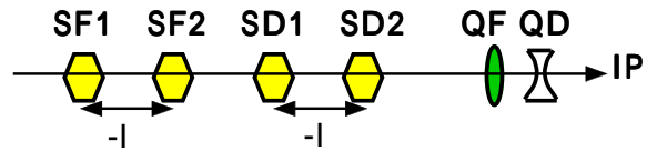
Figure 2: Cancellation of the Geometric Aberration
